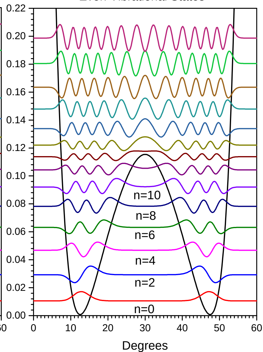
Even Vibrational States
