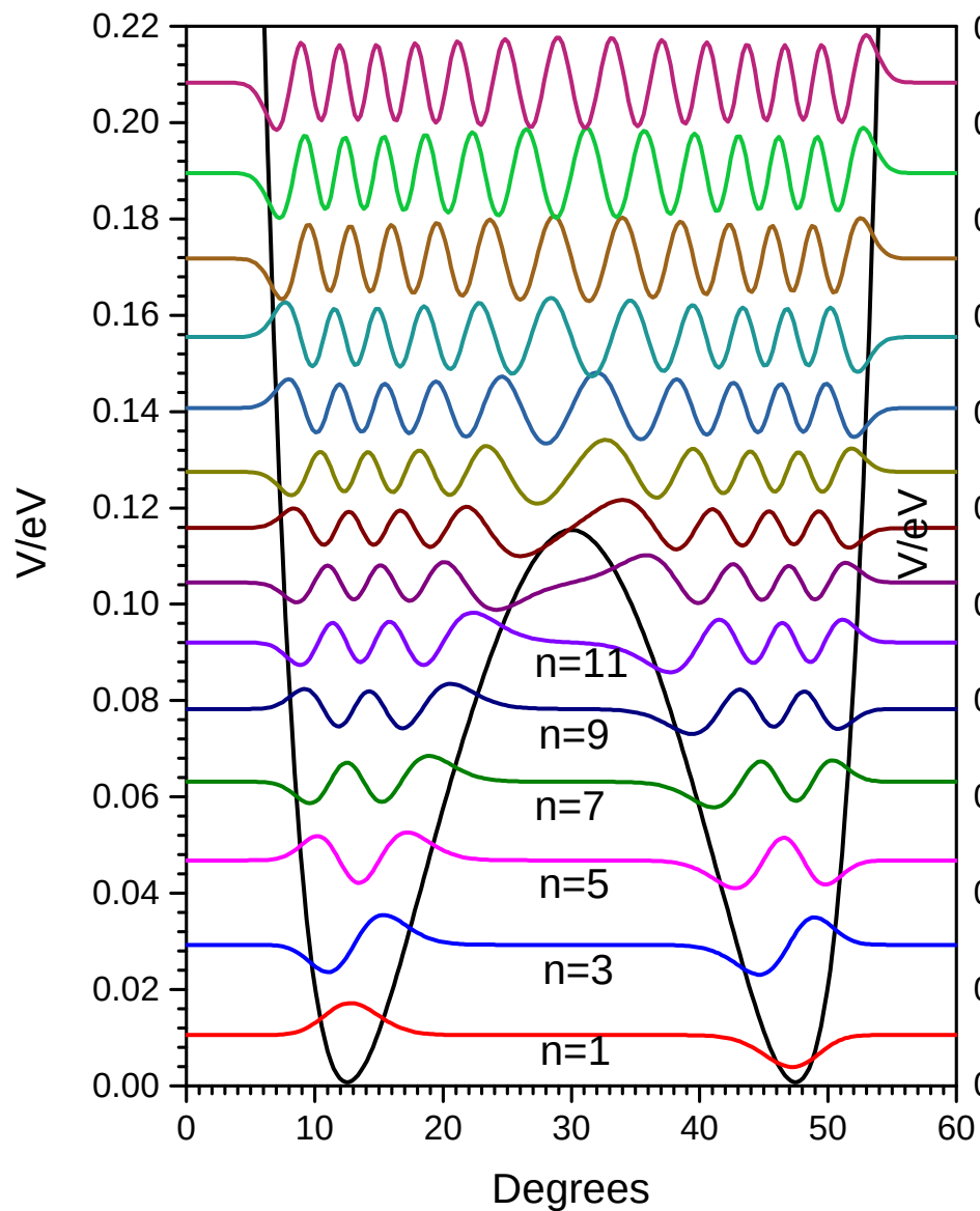
Odd Vibrational States
