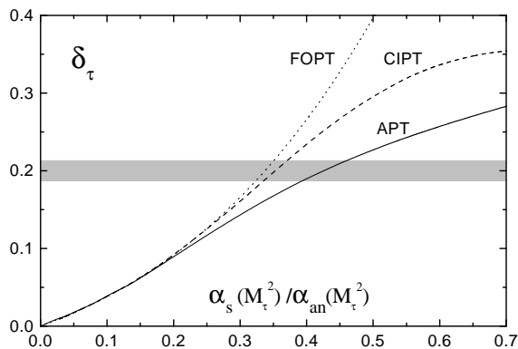
FIG. 1. Behavior of the QCD perturbative contribution to R_\tau as a function of \alpha_s(M_\tau^2) (for FOPT and CIPT) or of \alpha_{\text{an}}(M_\tau^2) (for APT) in the \overline{\text{MS}} renormalization scheme.
