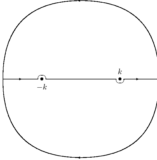
Figure 12.1: Contour in the k' plane used to evaluate the integral (12.110). The integral is closed in the upper (lower) half-plane if the exponent is positive (negative). The poles in the integrand are avoided by passing above the one on the left, and below the one on the right.
