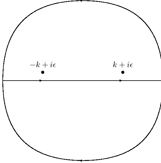
Figure 12.2: Contour in the \omega plane used to evaluate the integral (12.135).
