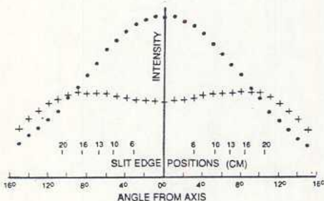
Fig. 2. Intensity of waves emitted from source horn as a function of the angle from the axis of the source horn. Solid dots are for the unmodified horn. Plus dots illustrate the effect of the vanes shown in Fig. 3. The scale of numbers from 6 to 20 indicates the edge positions of slits having various widths in centimeters. Intensity scale is arbitrary.
