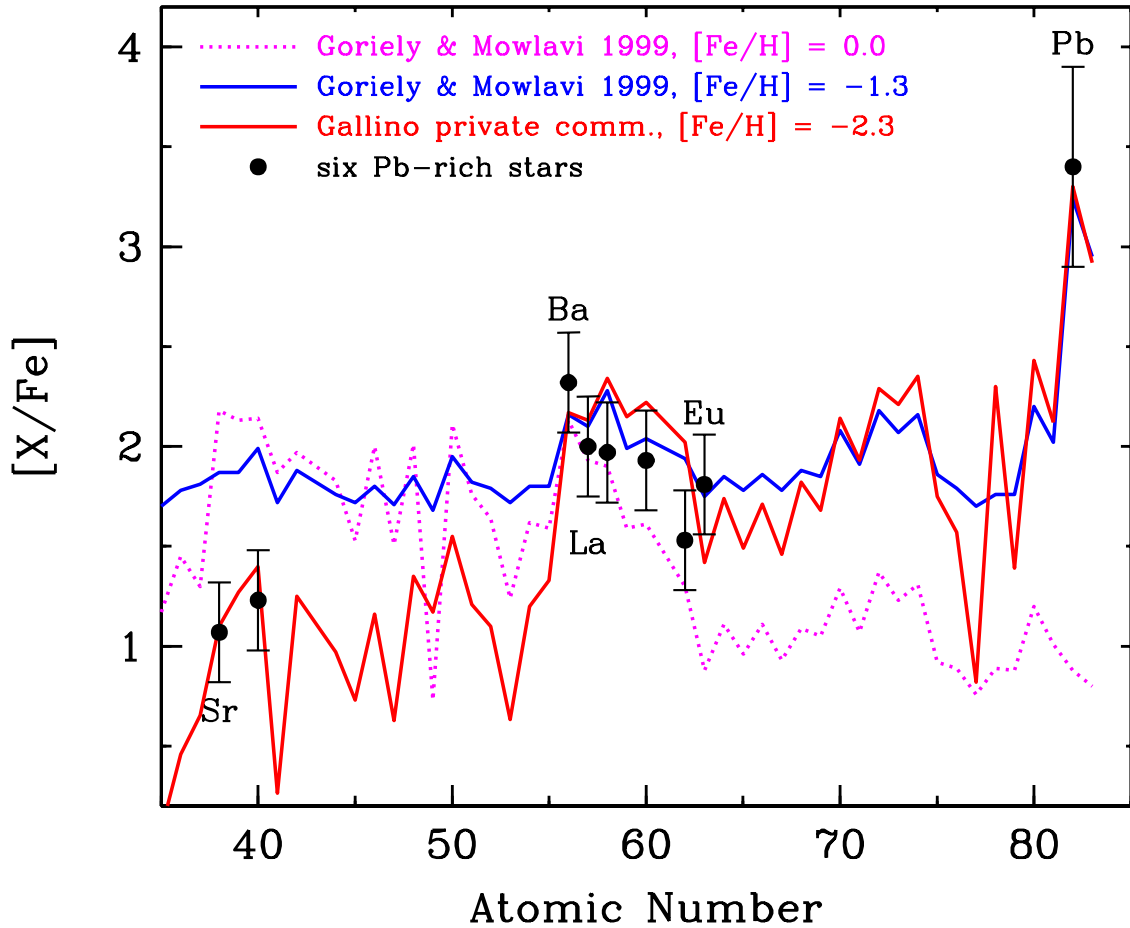
Fig. 8.— Comparison of the normalized mean n -capture abundances of the six Pb-rich metal-poor stars shown in the previous figure and abundance predictions of AGB star s -process nucleosynthesis (Goriely & Mowlavi 2000; Gallino, private communication). Lines and symbols are defined in the figure legend.
