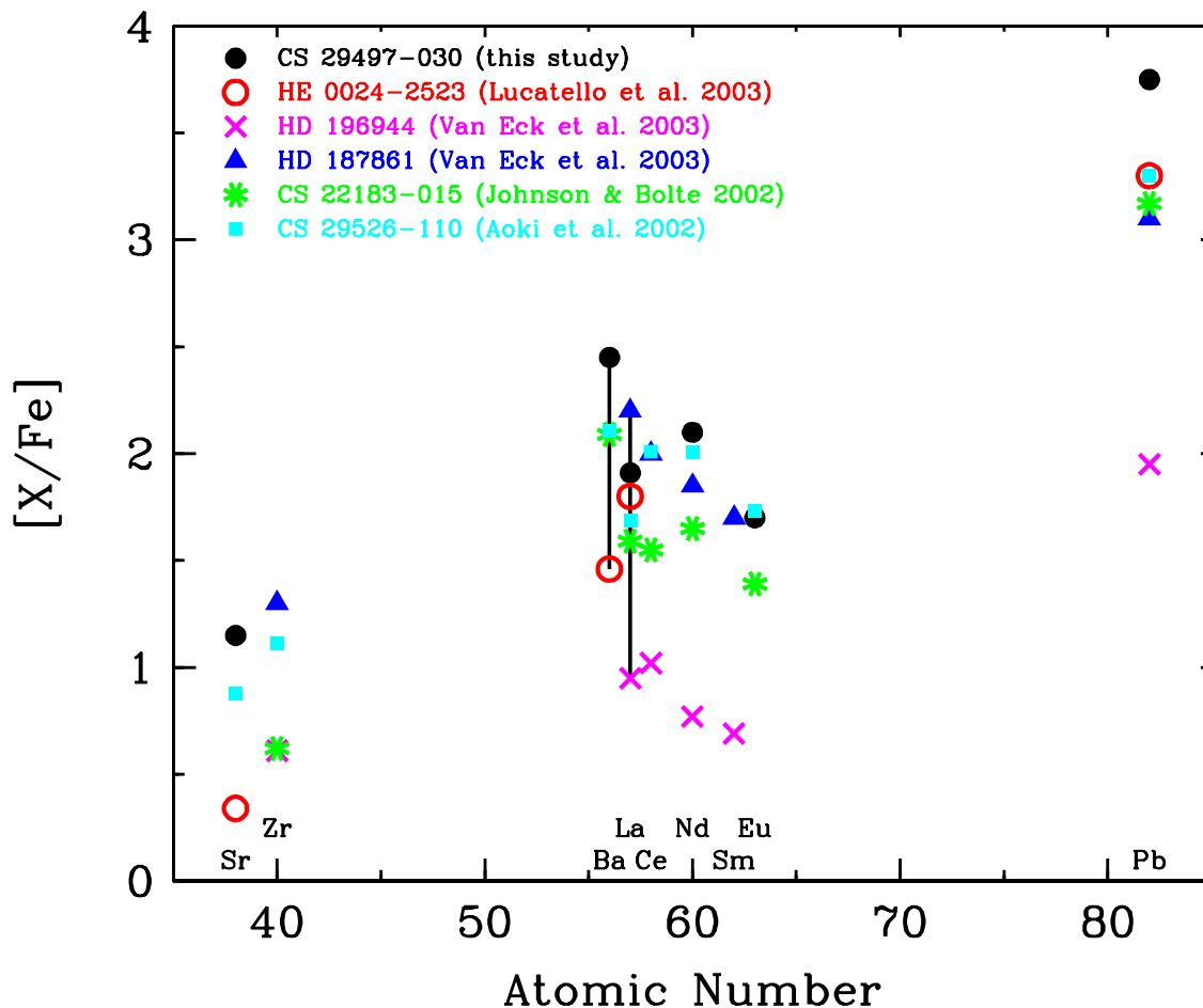
Fig. 7.— n -capture abundances in six extremely Pb-rich stars ( [Pb/(La \text{ or } Ba)] \gtrsim +1.0 ). The sources for the abundances are indicated in the figure legend. The vertical lines connecting the Ba and La abundances signify that mean abundances to be shown in the next figure have been computed after renormalization of the abundance sets from other studies to the observed Ba or La (or both) abundances of CS 29497-030.
