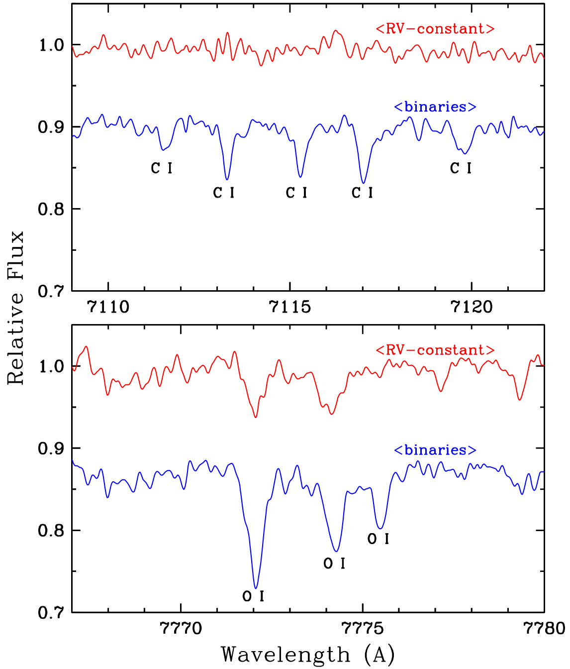
Fig. 4.— Spectra of C I and O I lines in the RV-constant and the binary BMP stars.
