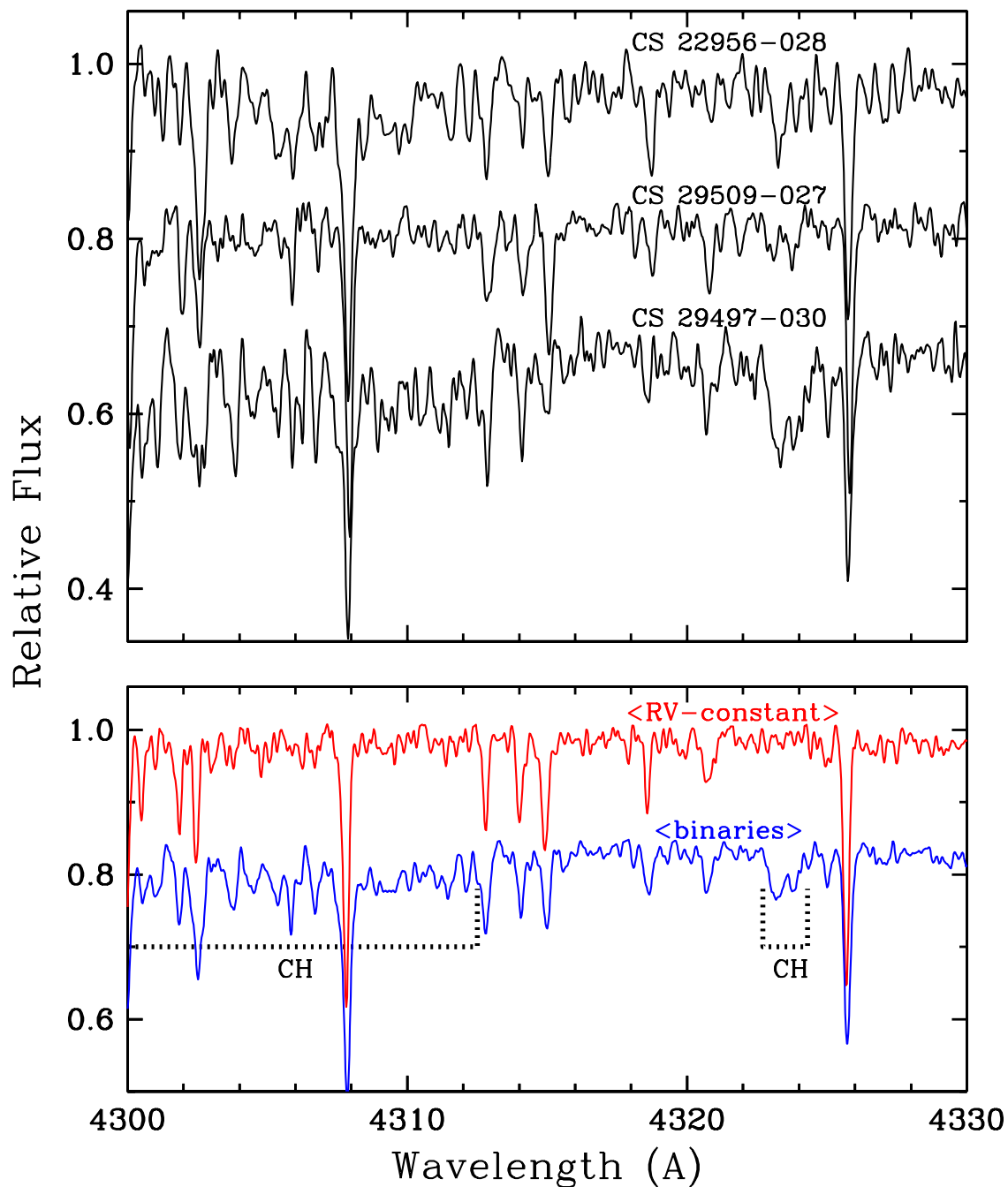
Fig. 3.— The CH G-band in the BMP program stars. In the upper panel, individual spectra of the three binaries are shown and in the lower panel the mean co-added spectra of the RV-constant stars (in this and other figures labeled <RV-constant>) and the binaries (labeled <binaries>) are shown. In each panel the relative flux scale of the top spectrum is correct and the other spectra are shifted downward by arbitrary additive amounts for display purposes. Regions of CH absorption are marked in the lower panel with dotted lines.
