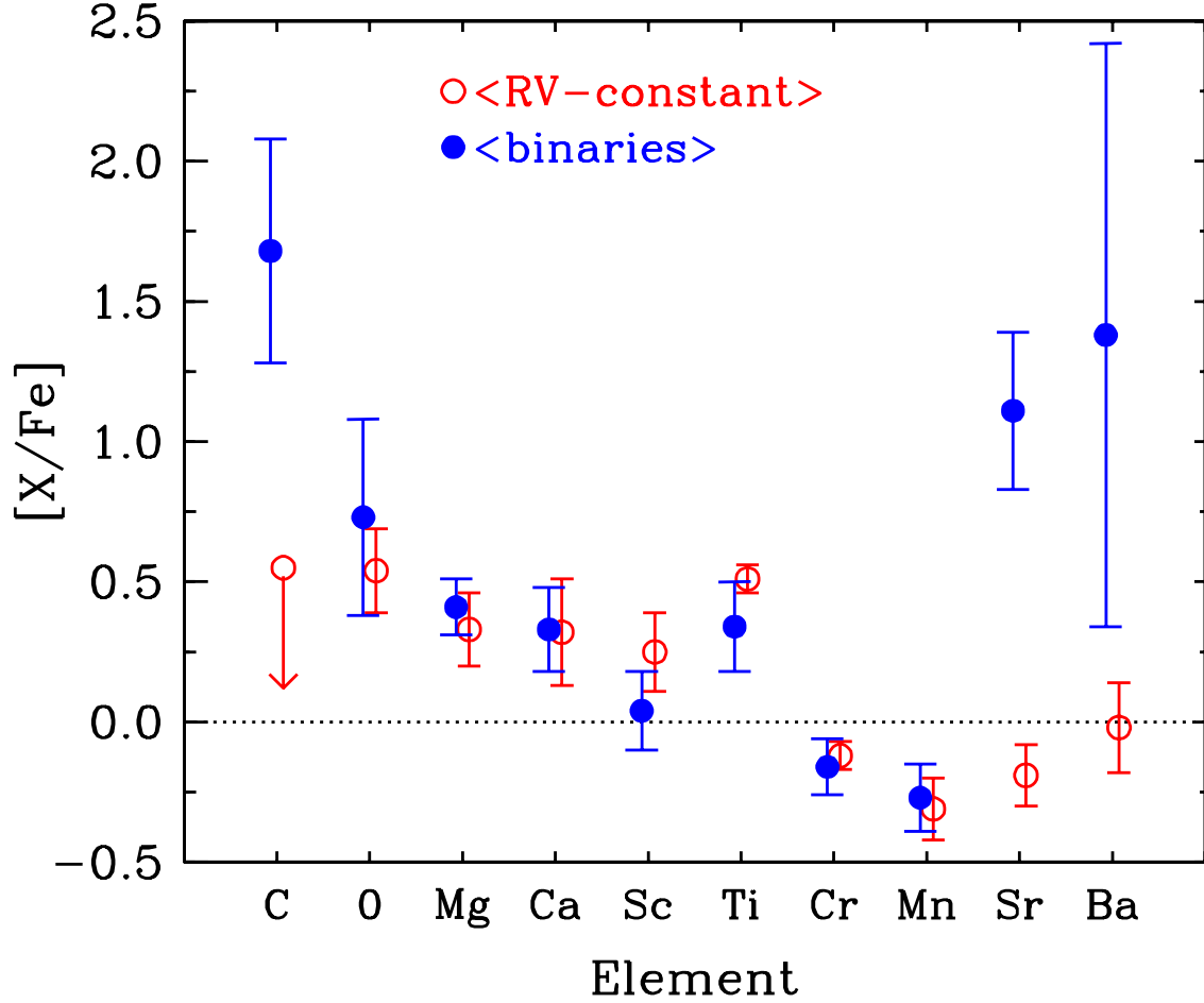
Fig. 5.— Average abundances of the BMP RV-constant and binary groups. Abundances of C, O, Sr, and Ba are from this paper, and those of the other elements are from PS00. Small horizontal shifts have been introduced to the points to the left for the binaries, and to the right for the RV-constant stars, for display purposes. Each abundance and its vertical range is the mean and the sample standard deviation \sigma of the values for each star in the group. The true observational/analytical uncertainties are typically about \pm 0.15 . Therefore the very large ranges for C, Sr, and Ba for the binaries represent true star-to-star scatter, far beyond abundance measurement errors.
