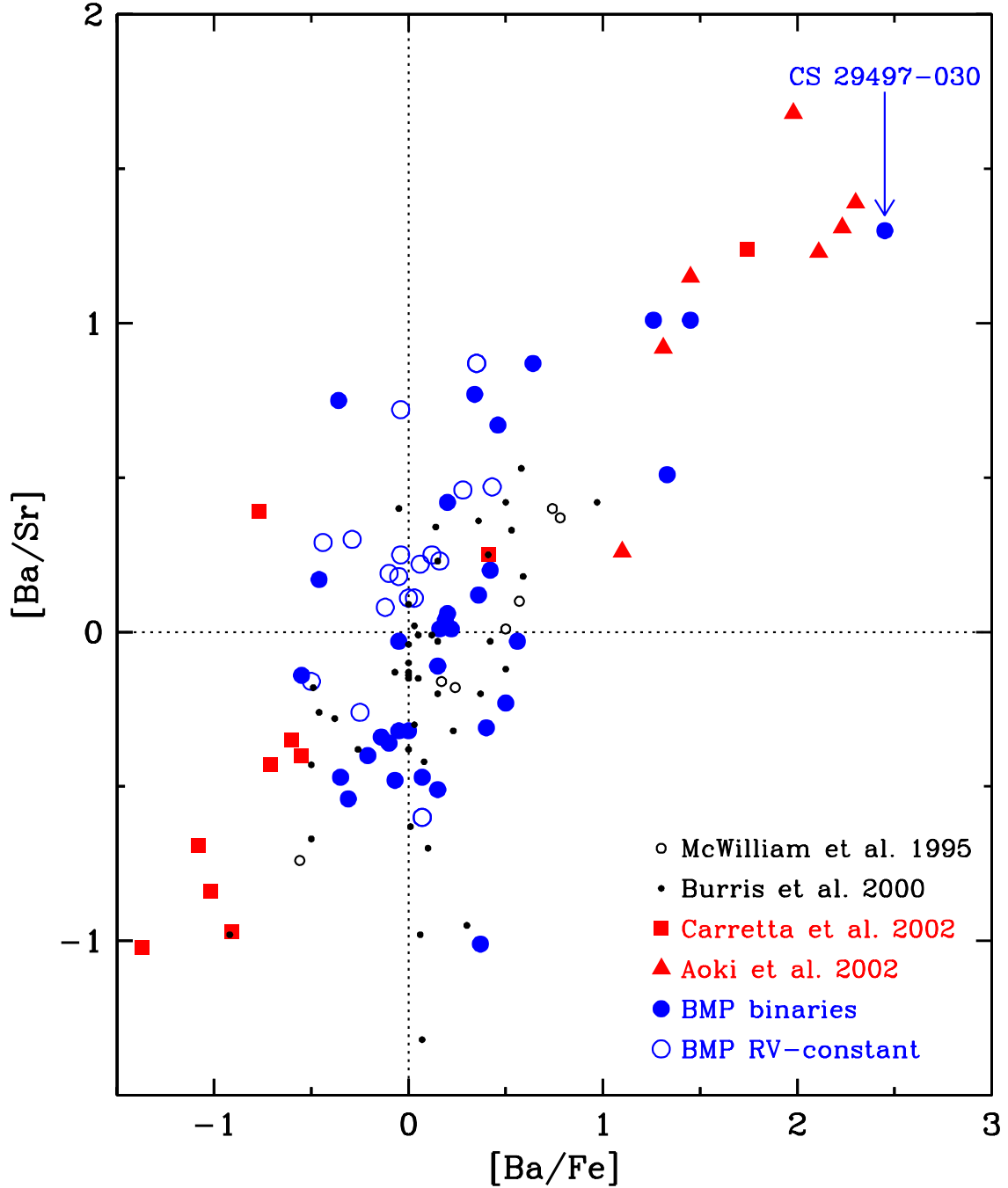
Fig. 9.— Correlation of [\text{Ba}/\text{Sr}] with [\text{Ba}/\text{Fe}] abundance ratios in metal-poor stars, combining results of several surveys. The horizontal and vertical dotted lines indicate solar ratios of [\text{Ba}/\text{Sr}] and [\text{Ba}/\text{Fe}] , respectively. The abundances for BMP RV-constant stars (large open circles) and binaries (large filled circles) are taken from this study and PS00. The McWilliam et al. (1995) and Burris et al. (2000) data are included because their large sample sizes are useful in showing the domain of this diagram covered by ordinary metal-poor stars. The Carretta et al. (2002) study includes one Pb-rich star. The Aoki et al. (2002) sample concentrated exclusively on s -process-rich stars. We exclude their star CS 22942-019, with its uncertain Sr abundance based on extremely strong Sr II lines.
