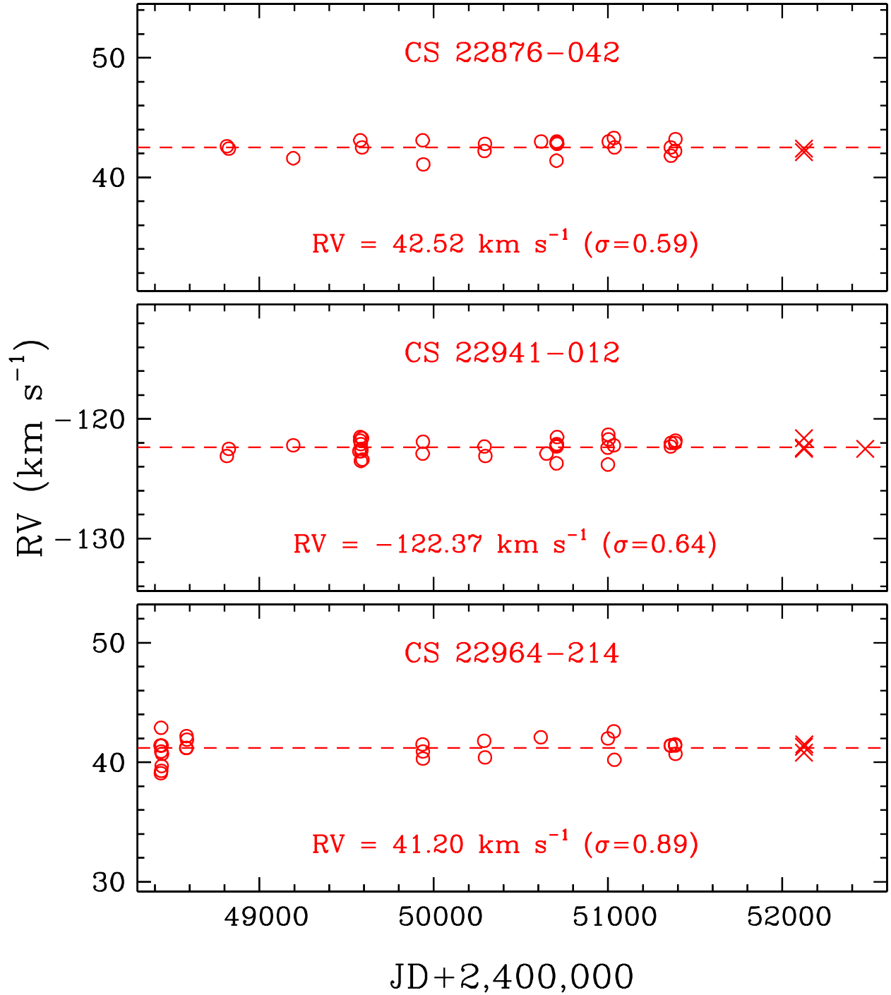
Fig. 1.— Velocities of the RV-constant stars as a function of Julian Date. The velocities from PS00 are shown as open circles, and the new velocities are shown as crosses. The vertical range in each panel of this and the next figure is 24 km s -1 .
