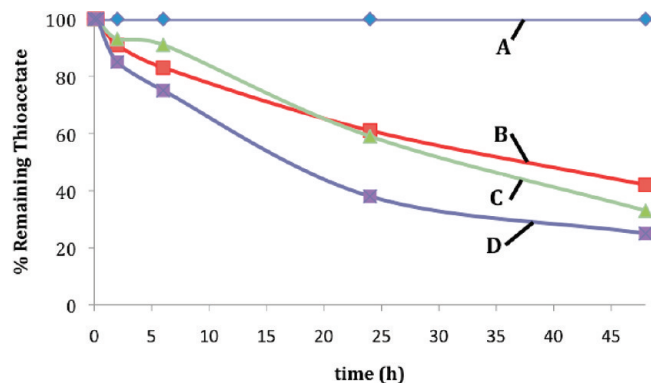
Figure 3. C10SAc (46 mM in \text{CD}_3\text{OD} ) cleavage by NMR monitoring. A: no additive. B: \text{NH}_4\text{OH} (115 mM). C: \text{HCl} (250 mM). D: propylamine (70 mM).
