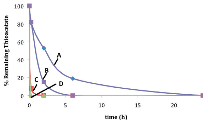
Figure 4. C10SAc (46 mM in \text{CD}_3\text{OD} ) cleavage by NMR monitoring. A: \text{K}_2\text{CO}_3 (46 mM). B: \text{NH}_4\text{OH} (575 mM). C: DBU (58 mM). D: KOH (58 mM).
