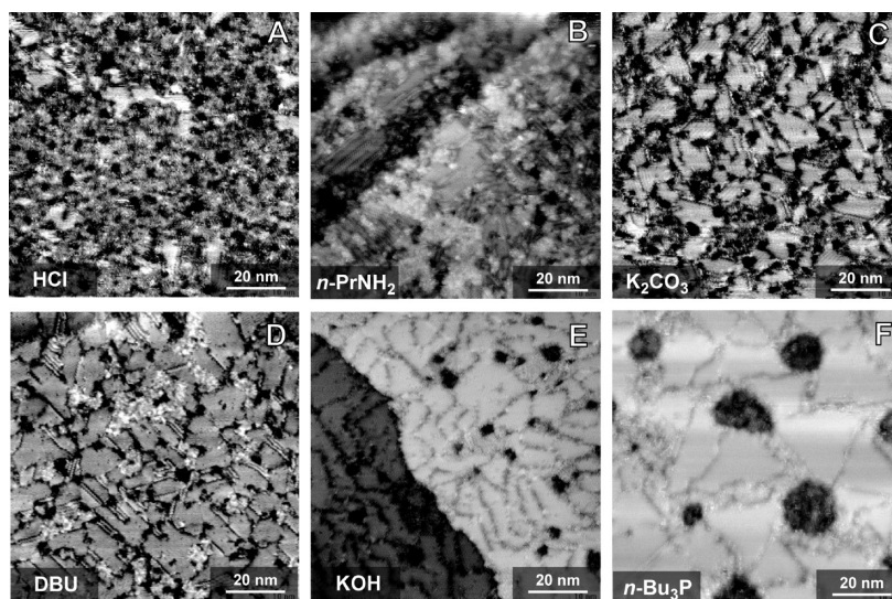
Figure 5. STM images SAMs on Au(111) grown for 16 h in 2.5 mM C10SAC in EtOH grown from a solution premixed for 1 h with 2.5 mM of (A) HCl, (B) \text{PrNH}_2 , (C) \text{K}_2\text{CO}_3 , (D) DBU, (E) KOH, and (F) \text{Bu}_3\text{P} . Each sample was grown from 2.5 mM each in ethanol (1 h premix, 16 h immersion of Au/mica). All STM images are 100 \text{ nm} \times 100 \text{ nm} . Tunneling conditions are V_{\text{sample}} = -1 \text{ V} and i_{\text{tunnel}} = 1 \text{ pA} . See text for details.
