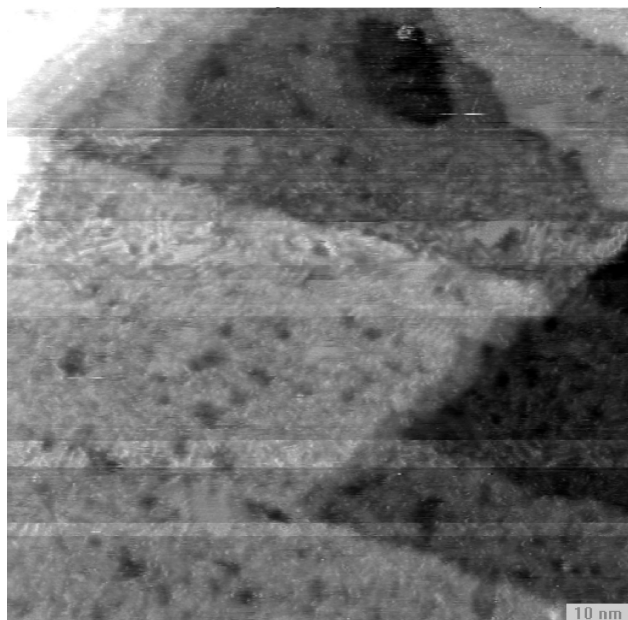
Figure 1. STM image of SAM on Au(111) grown for 16 h from C10SAc. The image is 100 nm \times 100 nm. Tunneling conditions are V_{\text{sample}} = -1 V and i_{\text{tunnel}} = 1 pA. See text for details.
