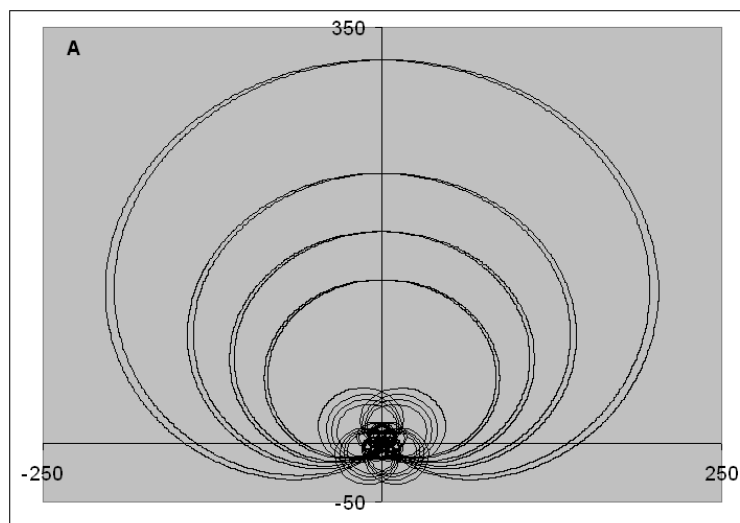
Figure 5. A classical trajectory in the complex- x plane for the complex Hamiltonian H = p^2 - (ix)^\pi . This complicated trajectory begins at x(0) = -7.1i and visits 11 sheets of the Riemann surface. Its period is approximately T = 255.3 . This figure displays the projection of the trajectory onto the principal sheet of the Riemann surface. Note that this trajectory does not cross itself.
