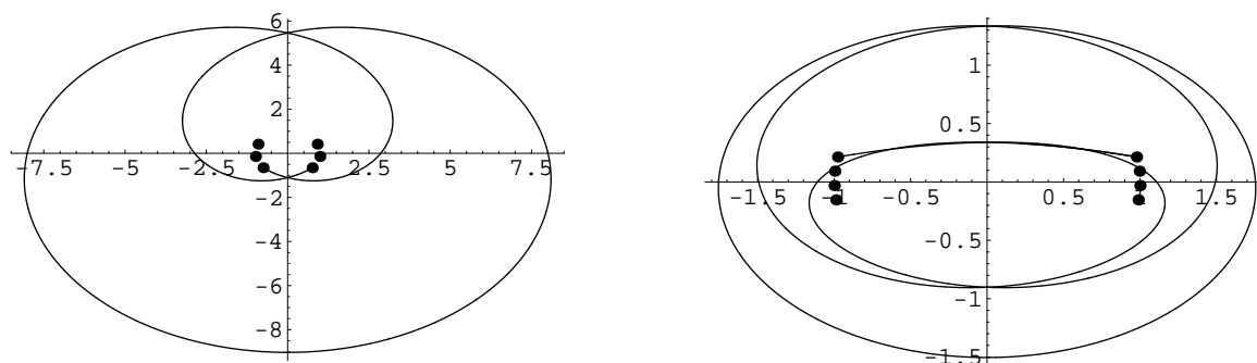
Figure 18. On the left the central orbit for \epsilon = 0.2 terminating at the n = 2 pair of turning points. This orbit crosses the imaginary axis 5 times. On the right the central orbit for \epsilon = 0.04 terminating at the n = 3 pair of turning points. This orbit crosses the imaginary axis 7 times.
