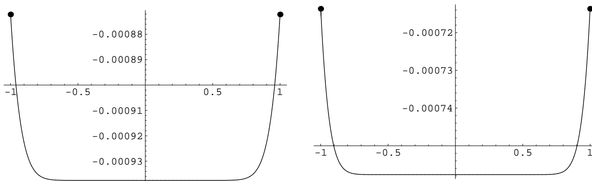
Figure 33. On the left, central orbit terminating at the n = 4 pair of turning points for \epsilon = 16.01 . On the right, central orbit terminating at the n = 5 pair of turning points for \epsilon = 20.01 .
