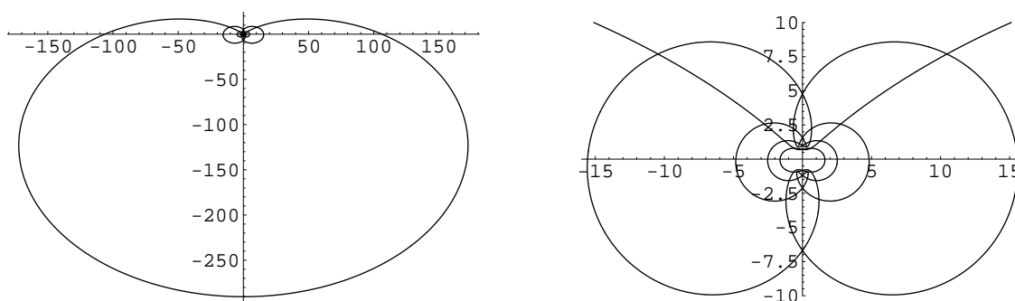
Figure 31. Central orbit for \epsilon = 1.305 terminating at the n = 1 pair of turning points. This orbit crosses the imaginary axis 17 times. On the principal sheet the central orbit resembles a large cardioid having a horizontal extent of over 300. To the right is a detail of the region near the origin.
