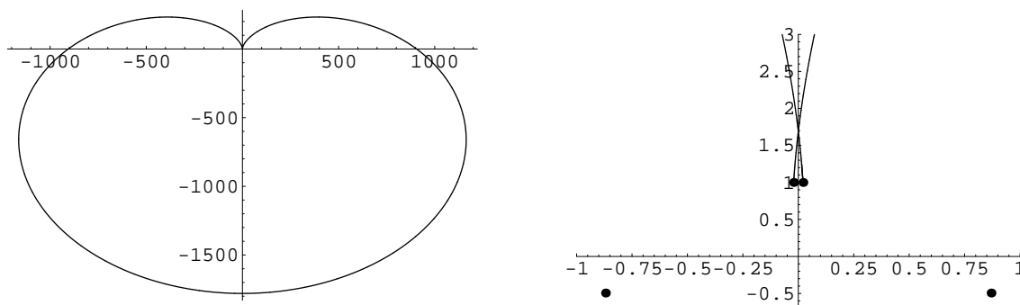
Figure 20. On the left the central orbit for \epsilon = 0.98 terminating at the n = 1 pair of turning points. This orbit crosses the imaginary axis 3 times. Note that this orbit is huge and that its shape resembles a cardioid. Our numerical studies indicate that as \epsilon tends to 1, the size of the orbit becomes infinite. On the right is an enlargement showing the detail near the origin.
