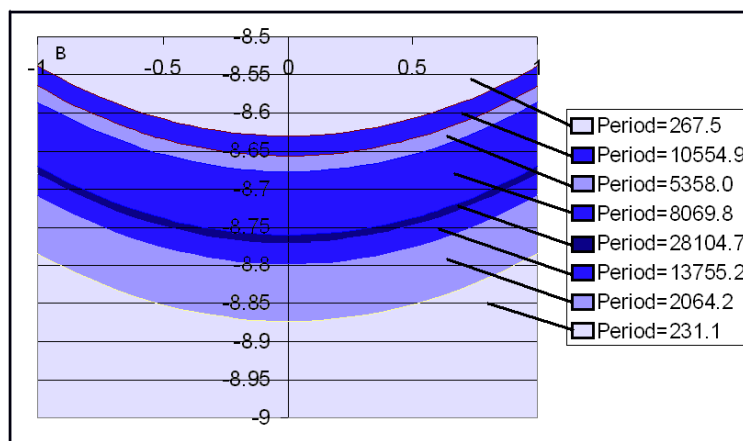
Figure 8. A small portion of the complex- x plane showing the dependence of the periods T of the classical orbits on the choice of initial condition x(0) for the case \epsilon = \pi - 2 . Note that T is extremely sensitive to the value of x(0) . There is an unresolved region between the band corresponding to T = 28,104.7 and T = 13,755.2 . We conjecture that arbitrarily long periods can be found in arbitrarily thin regions between x(0) = -8.767i and x(0) = -8.770i .
