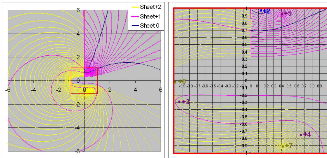
Figure 11. The classical orbit in the complex- x plane corresponding to Fig. 10. The oscillation in Fig. 10 corresponds to nested U-turns around a turning point in the complex plane.
