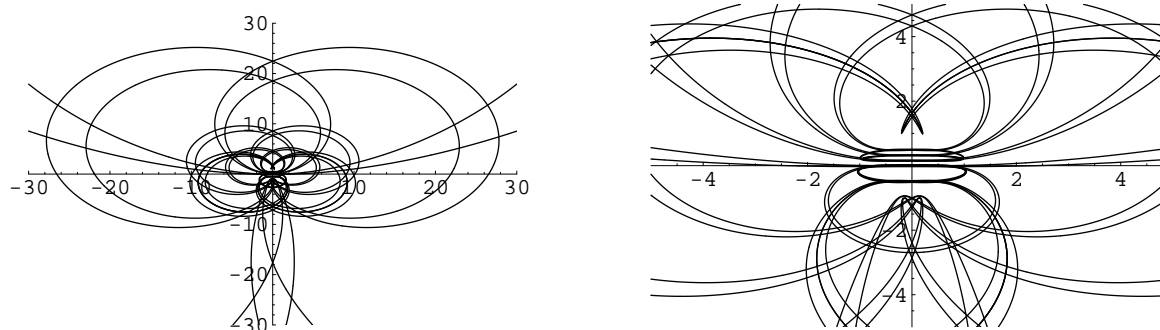
Figure 29. Two enlargements of the n = 1 central orbit for \epsilon = 1.2115214 in Fig. 28 (right). By careful examination of these detailed graphs, one can determine that the crossing number is K = 69 .
