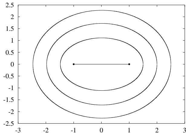
Figure 1. Classical trajectories in the complex- x plane for the harmonic oscillator whose Hamiltonian is H = p^2 + x^2 . These trajectories represent the possible paths of a particle whose energy is E = 1 . The trajectories are nested ellipses with foci located at the turning points at x = \pm 1 . The real line segment (degenerate ellipse) connecting the turning points is the usual periodic classical solution to the harmonic oscillator. All closed paths have the same period \pi by virtue of Cauchy's integral theorem.
