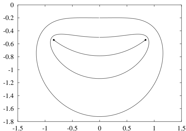
Figure 2. Classical trajectories in the complex- x plane for the complex oscillator whose Hamiltonian is H = p^2 - (ix)^\pi , which is (1) with \epsilon = \pi - 2 . As in Fig. 1 the trajectories represent the possible paths of a particle whose energy is E = 1 . The trajectories are deformed versions of the ellipses in Fig. 1. By virtue of Cauchy's integral theorem all of the closed trajectories have the same period T as given in (5).
