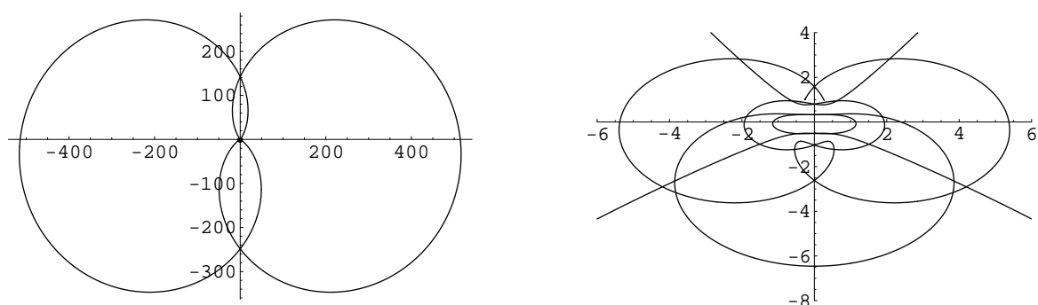
Figure 30. Central orbit for \epsilon = 1.286 terminating at the n = 1 pair of turning points. This orbit crosses the imaginary axis 17 times. The central orbit is dominated by a huge double-cardioid structure having a horizontal extent of over 1000. This structure lies on the \pm 1 sheets of the Riemann surface. To the right is a detail of the region near the origin.
