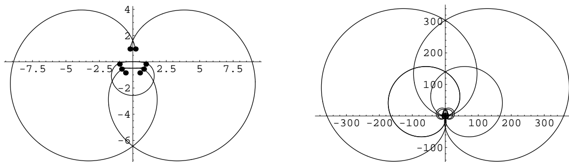
Figure 28. Transition between a K = 9 orbit (left) and a K = 69 orbit (right). The left graph shows a central n = 1 orbit that corresponds to \epsilon = 1.2115215 and the right graph shows a central n = 1 orbit that corresponds to \epsilon = 1.2115214 . It is not easy to see that the right orbit actually crosses the imaginary axis 69 times, so the region of this orbit near the origin is displayed in Fig. 29.
