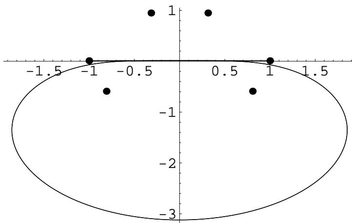
Figure 19. Central orbit for \epsilon = 1.34 terminating at the n = 2 pair of turning points. This orbit crosses the imaginary axis 3 times. This orbit does not enclose the n = 1 turning points.
