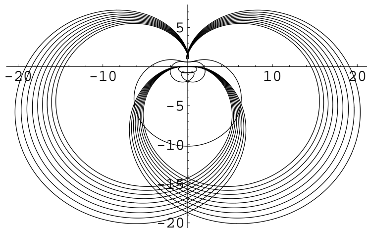
Figure 24. Central orbit for \epsilon = 1.14745 terminating at the n = 1 pair of turning points. This orbit crosses the imaginary axis 61 times.
