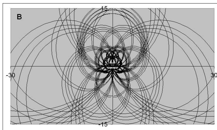
Figure 6. An enlargement of the classical trajectory x(t) in Fig. 5 showing the detail near the origin in the complex- x plane. We emphasize that this classical path never crosses itself; the apparent self-intersections are paths that lie on different sheets of the Riemann surface.
