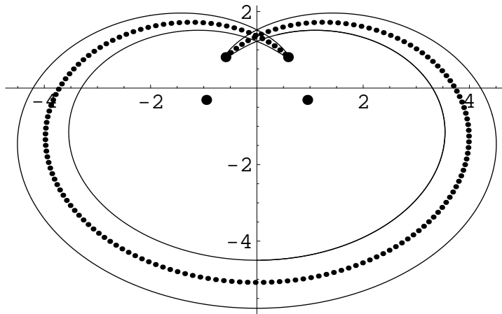
Figure 12. Two orbits for \epsilon = 0.5 that have the same period. The solid-line orbit encircles the turning points. The dashed-line orbit is the central orbit that terminates at the n = 1 pair of turning points. The n = 0 and n = 1 pairs of turning points are indicated by dots. The period of this class of orbits is T = 5.54559 .
