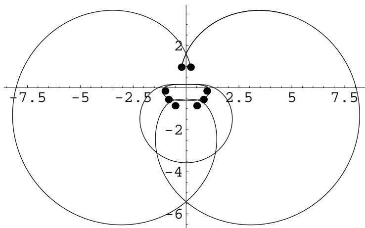
Figure 14. Central orbit for \epsilon = 1.225 terminating at the n = 1 pair of turning points. This orbit crosses the imaginary axis 9 times.
