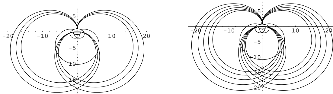
Figure 22. Second transition between two topological classes of graphs. The left graph shows the central orbit for \epsilon = 1.1478263 terminating at the n = 1 pair of turning points. This orbit crosses the imaginary axis 25 times. The right graph shows the central orbit for \epsilon = 1.1478262 terminating at the n = 1 pair of turning points. This orbit crosses the imaginary axis 37 times.
