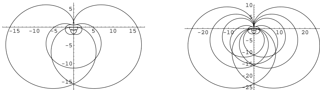
Figure 21. Transition between two topological classes of graphs. The left graph shows the central orbit for \epsilon = 1.149739 terminating at the n = 1 pair of turning points. This orbit crosses the imaginary axis 13 times. The right graph displays the central orbit for \epsilon = 1.149738 terminating at the n = 1 pair of turning points. This orbit crosses the imaginary axis 25 times.
