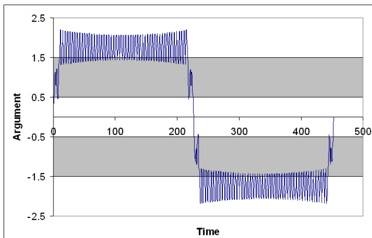
Figure 10. The argument of the classical orbit as a function of time t for \epsilon = \pi - 2 and initial condition x(0) = -17i . This orbit has period T = 452.6 and visits 5 sheets of the Riemann surface. Note the persistent oscillation in the classical orbit.
