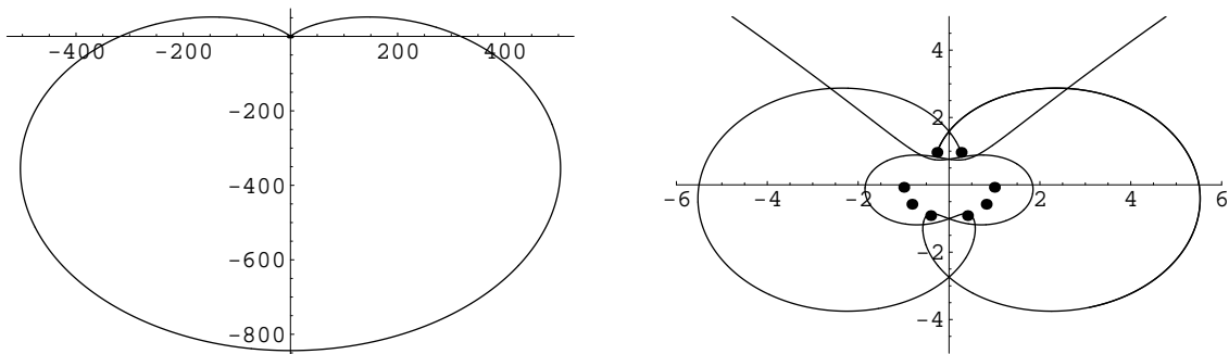
Figure 27. Central orbit for \epsilon = 1.282 terminating at the n = 1 pair of turning points. This orbit crosses the imaginary axis 9 times. To the right is a detail of the region near the origin.
