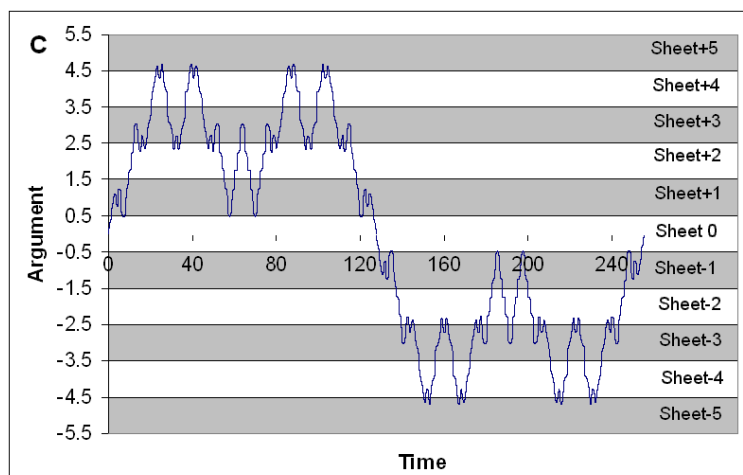
Figure 7. The argument (complex phase) of the classical orbit shown in Figs. 5 and 6 plotted as a function of time for one complete cycle. The period of this cycle is T = 255.3 . The classical particle starts on the negative imaginary axis on sheet 0 where the phase is defined to be 0. The particle then visits 11 sheets of the Riemann surface from sheet -5 to sheet 5 .
