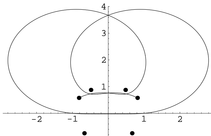
Figure 16. Central orbit for \epsilon = 2.31 terminating at the n = 1 pair of turning points. This orbit crosses the imaginary axis 5 times. Note that this orbit does not enclose the n = 0 turning points.
