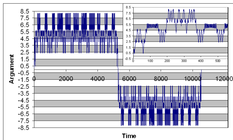
Figure 9. The argument of a long-period classical orbit for which \epsilon = \pi - 2 and the initial condition is x(0) = -8.63026i . This orbit has period T = 10,554.9 and visits 17 sheets of the Riemann surface. Note the oscillatory fine structure of this orbit in the inset.
