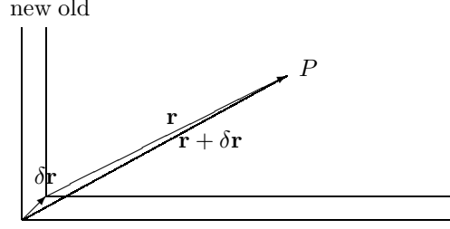
Figure 1.1: Description of a physical point P in two different coordinate systems, labeled “old” and “new,” that differ by a displacement \delta \mathbf{r} .
